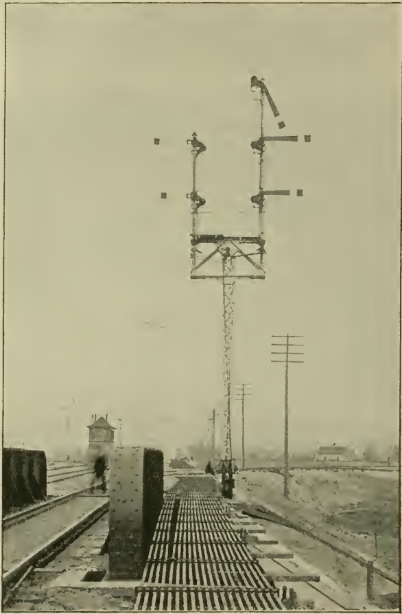
RAILWAY SIGNALS.
